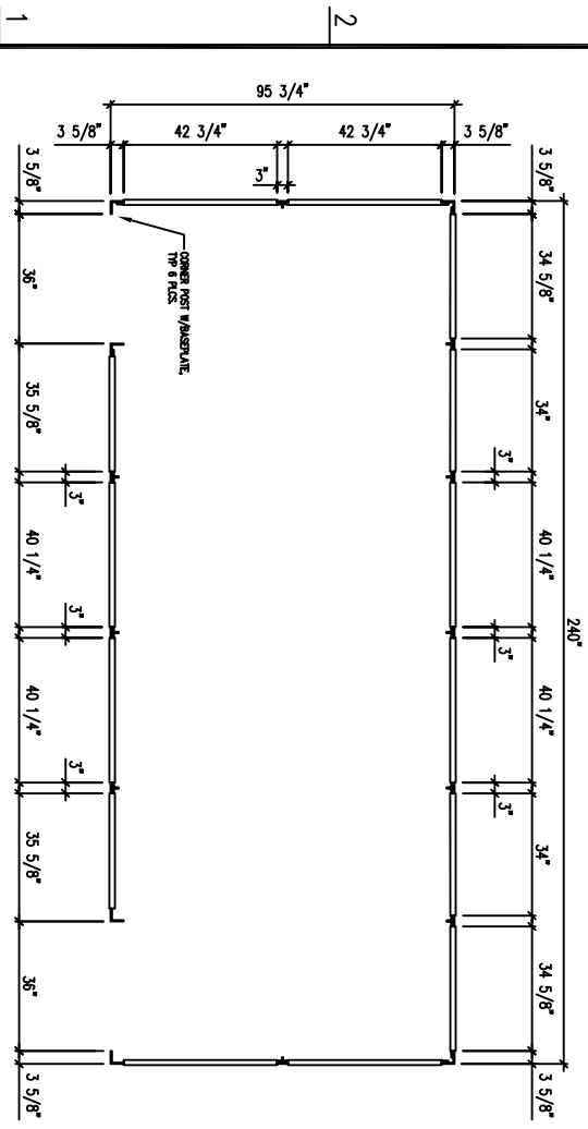
STYLE 'C' FLOOR PLAN
