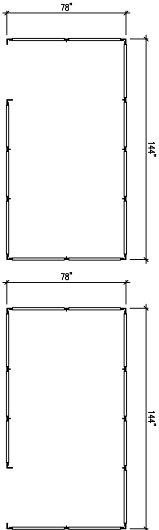
STYLE 'A' FLOOR PLAN
