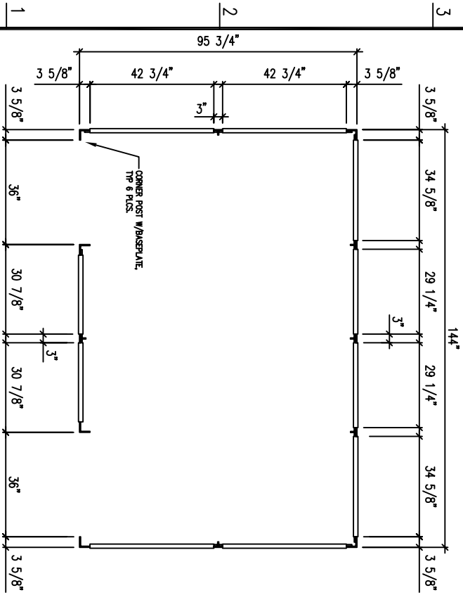
STYLE 'C' FLOOR PLAN
