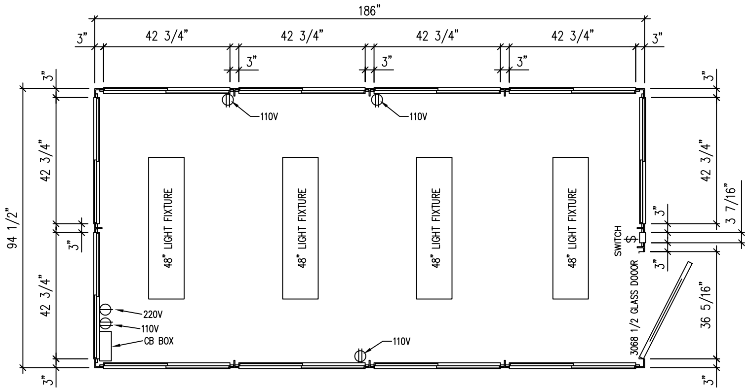
FLOOR PLAN
