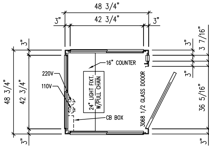
FLOOR PLAN
