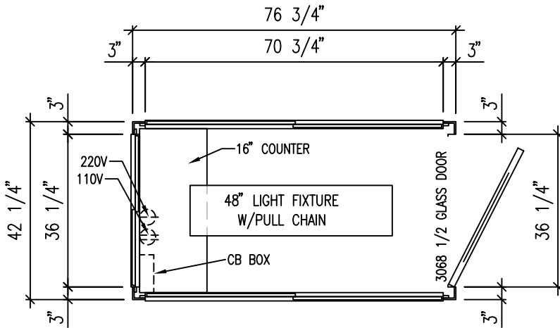
FLOOR PLAN
