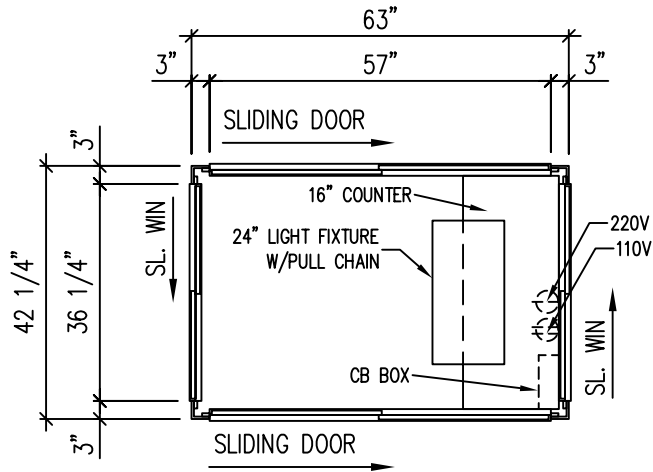
FLOOR PLAN
