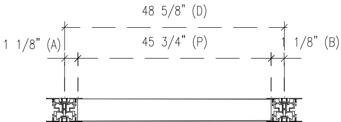
Stud to Stud Dimension P = D - (A + B)
