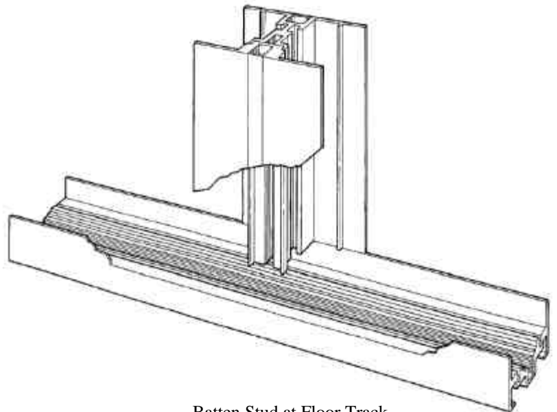
Batten Stud at Floor Track
