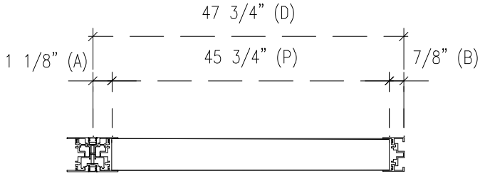
Stud to Wall Starter Dimension P = D - (A + B)
