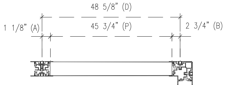
Stud to Corner Dimension P = D - (A + B)
