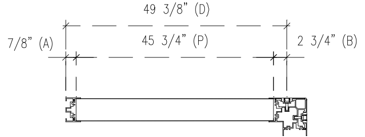
Wall Starter to Corner Dimension P = D - (A + B)
