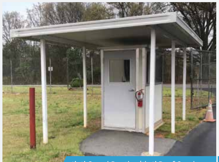
4'x4' Guard Booth with 4' Roof Overhang
