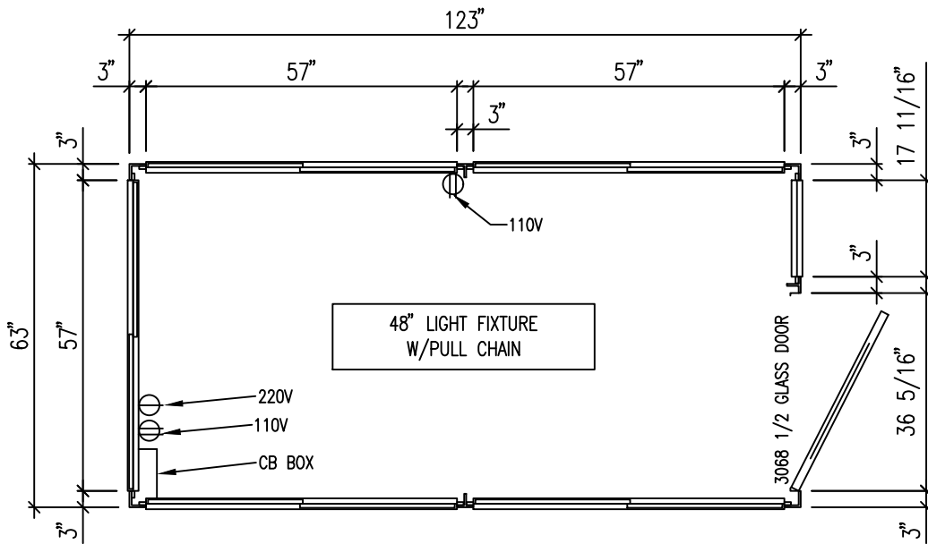
FLOOR PLAN
