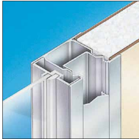
Window-stud-panel detail.
